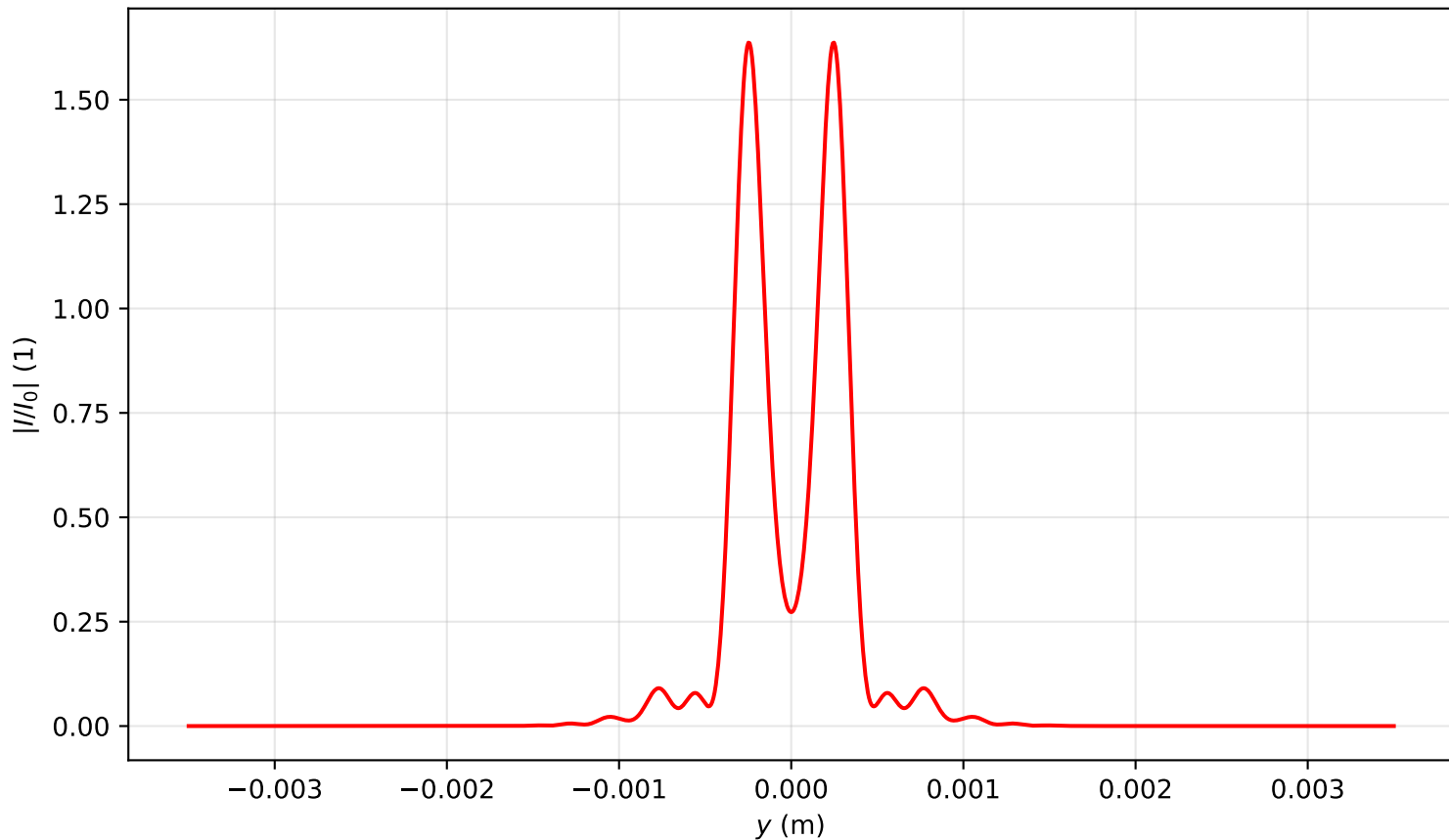
Intensity profile I(x=0, y, z=1.194)/I_0 , P_{in}=2.5P_{cr} , artificial time
